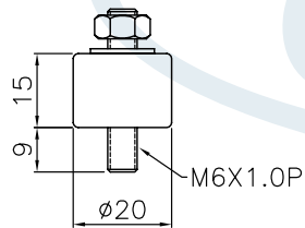
Shock Resistant 避震橡腳
