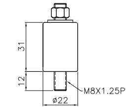
Shock Resistant 避震橡腳
